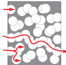
Figure 1. Good Porosity but Poor Permeability.
